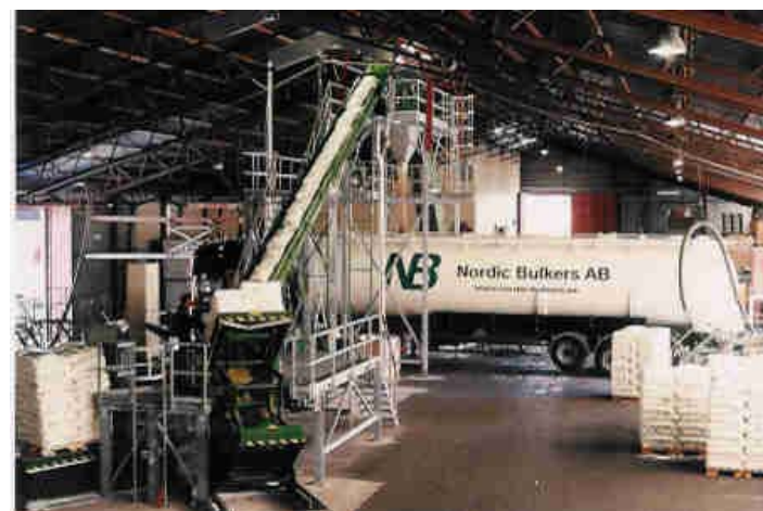
Semi-automatic bag slitting installation, Wallhamn
